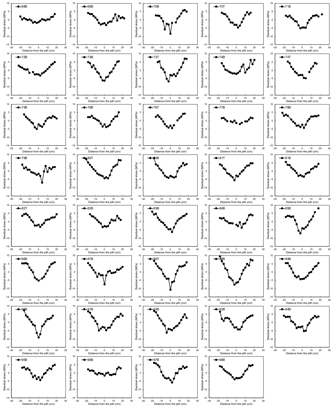
Fig. 6 Radial distribution of residual stress for each board (log no. 68-98, T: board from a top-end log, B: board from a butt-end log)
