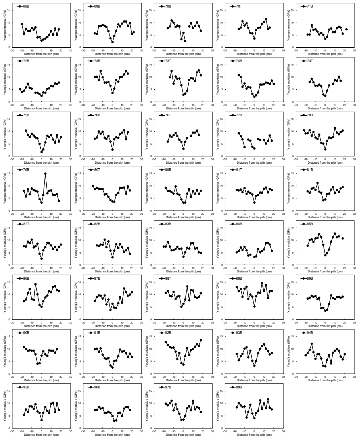
Fig. 4 Radial distribution of Young's modulus for each board (log no. 68-98, T: board from a top-end log, B: board from a butt-end log)
