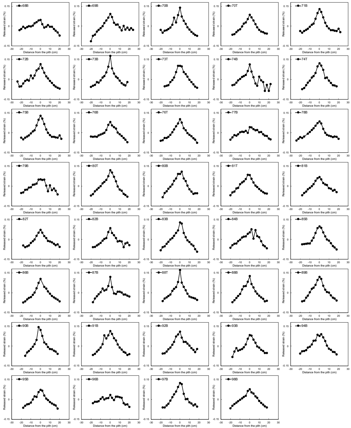
Fig. 2 Radial distribution of released strain for each board (log no. 68-98, T: board from a top-end log, B: board from a butt-end log)
