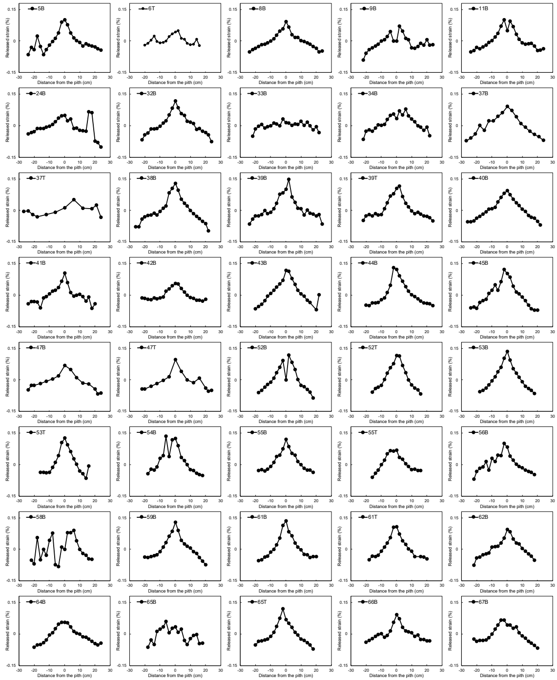
Fig. 1 Radial distribution of released strain for each board (log no. 5-67, T: board from a top-end log, B: board from a butt-end log)
