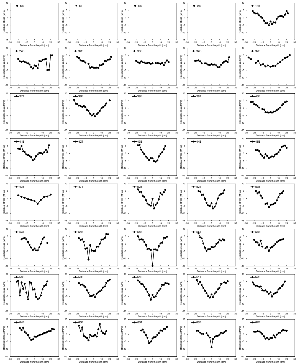
Fig. 5 Radial distribution of residual stress for each board (log no. 5-67, T: board from a top-end log, B: board from a butt-end log, blank graph: not measured)
