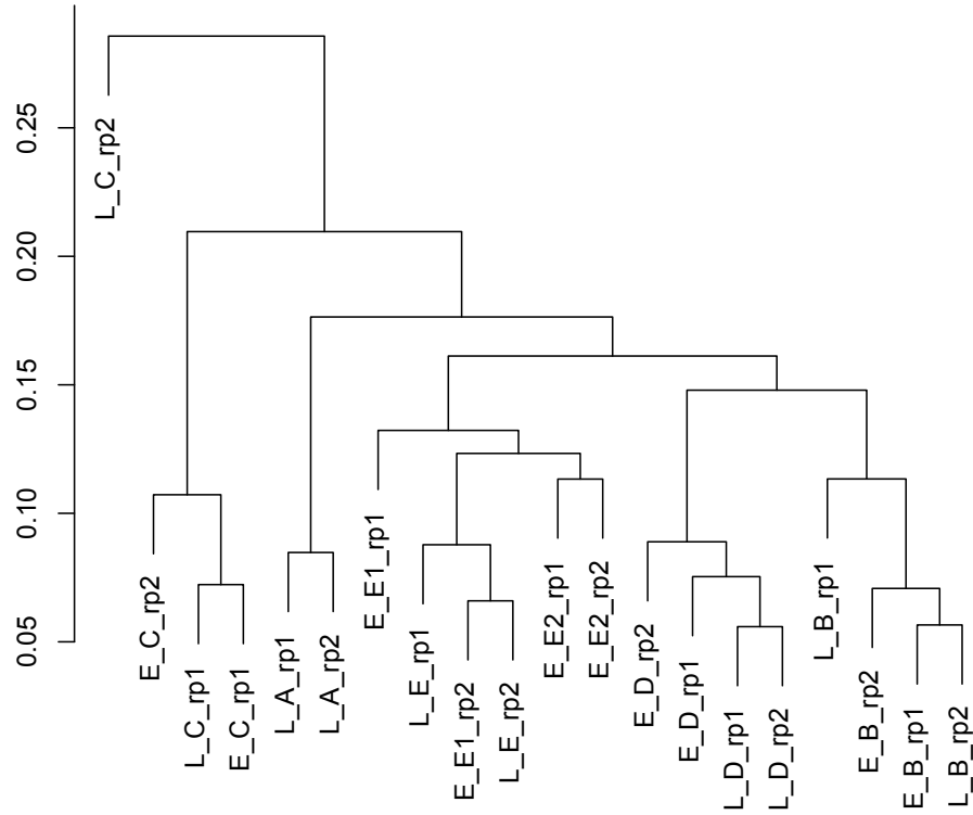
Fig. S2. Hierarchical clustering of all samples based on the expression pattern of the transcripts. Prefix denotes CO 2 conditions, and the suffix indicates the replicate number (rp1 or rp2).
