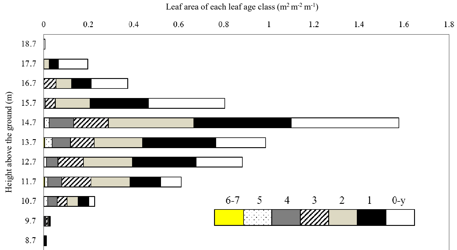
Supplementary Fig. 1. Vertical distribution of leaf area of each leaf age class in the 33-year-old Cryptomeria japonica var. japonica forest canopy in the Kunugidaira PSP
