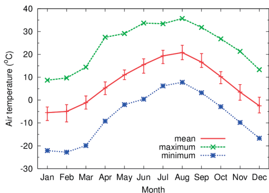
Fig. 1. 気温の季節変化 実線は観測期間中の各月の欠測が 10% 未満の月の平均値およびエラーバーは月平均値の最高・最低値。破線は観測期間中の各月の最高気温、点線は最低気温。 Seasonal variation in air temperature Solid line and error bars show the average and maximum/minimum monthly means of each month. Monthly data sets with less than 10% data gap were used for statistics. Dashed and dotted lines show the maximum and the minimum values for all observation periods of each month.
